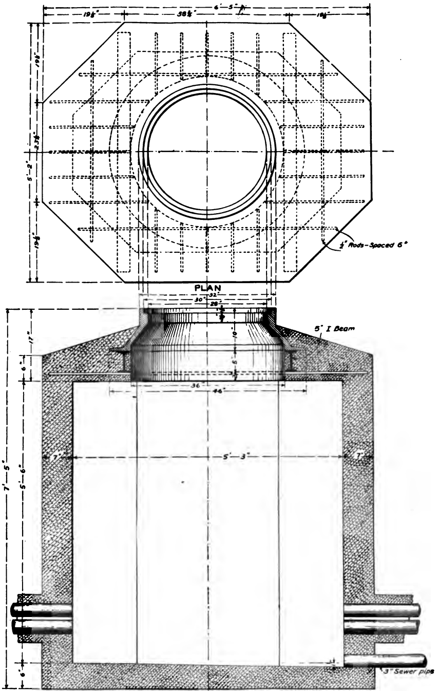
SECTION OF MANHOLE
